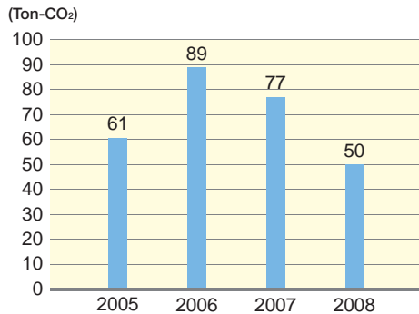
Shift of Generation of Energy-Oriented CO 2
